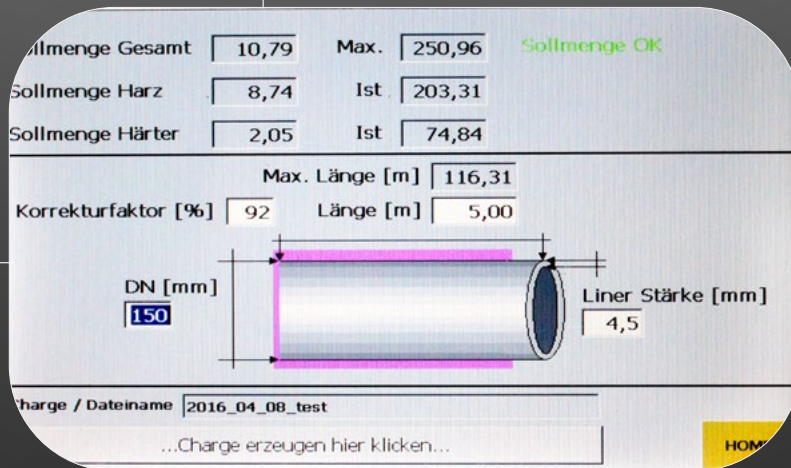
SPS control system
