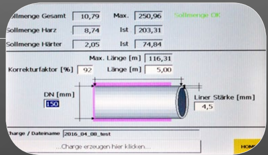
SPS control
